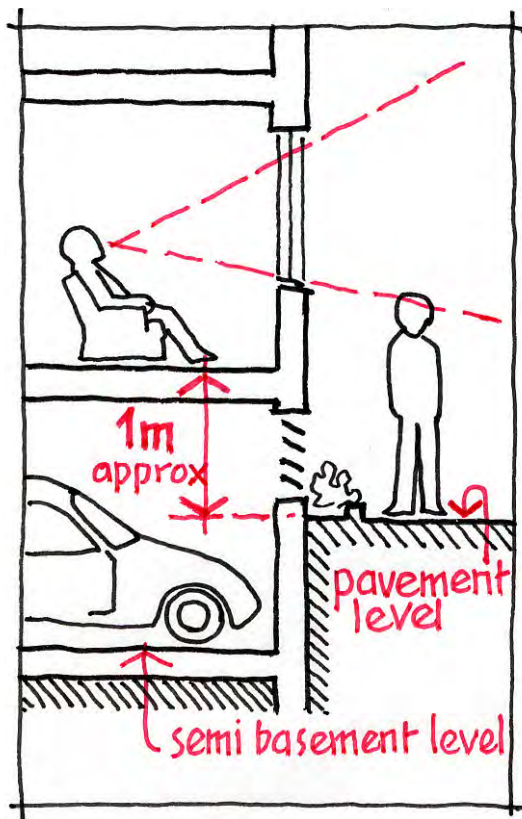
Figure 5.21 Garages
