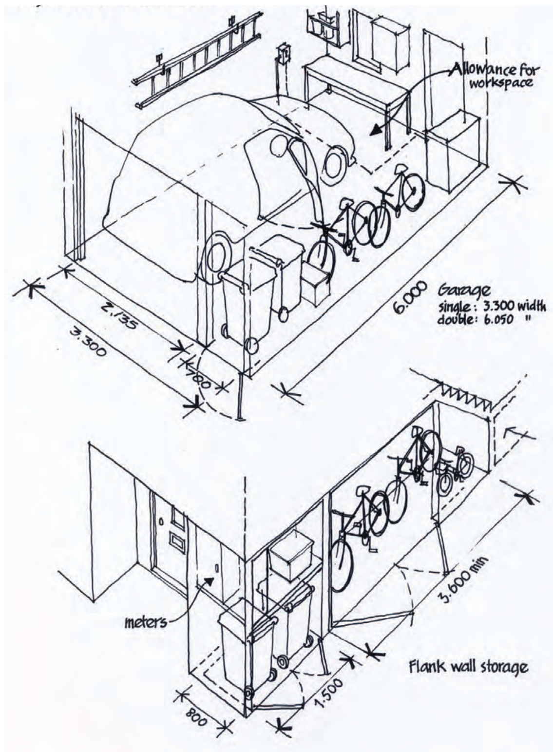
Figure 5.22 Storage - Residential
