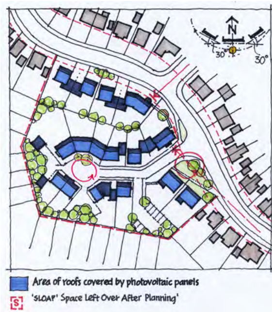
Figure 5.2 Layout - 30° option
