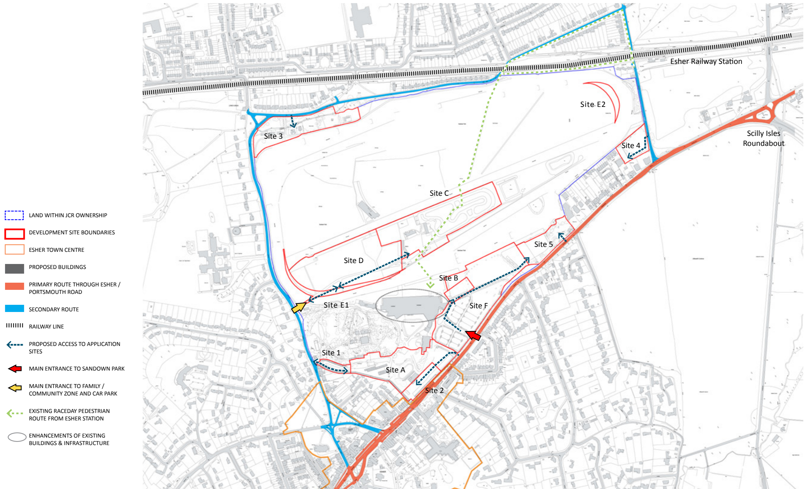
Fig. 4: Masterplan Access and Movement Diagram
