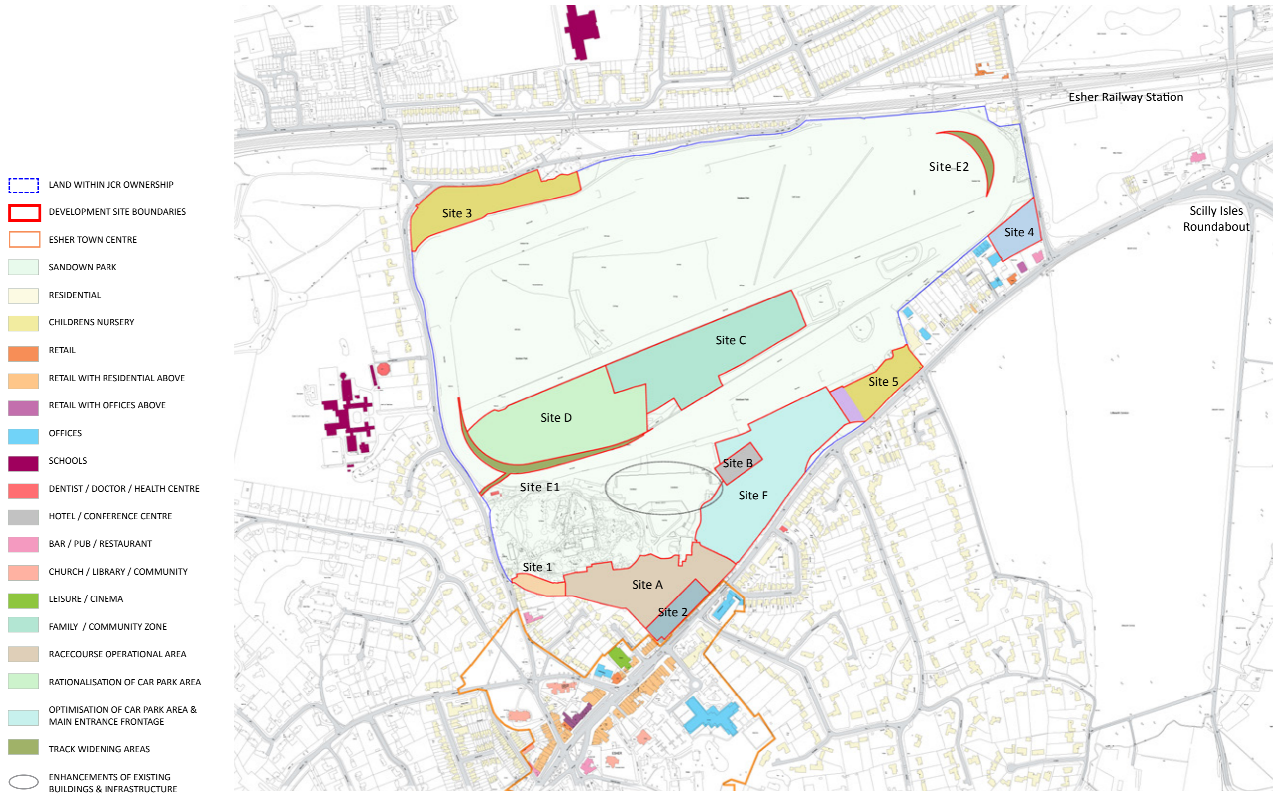
Fig. 3: Masterplan Land Uses Diagram
