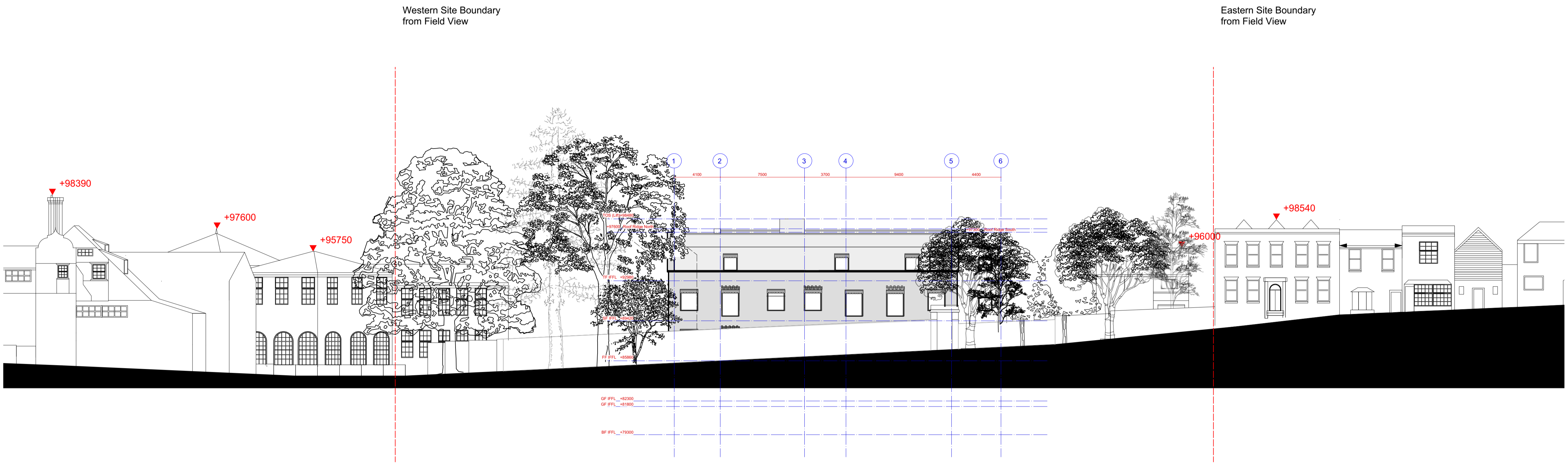
Elevation - South A
