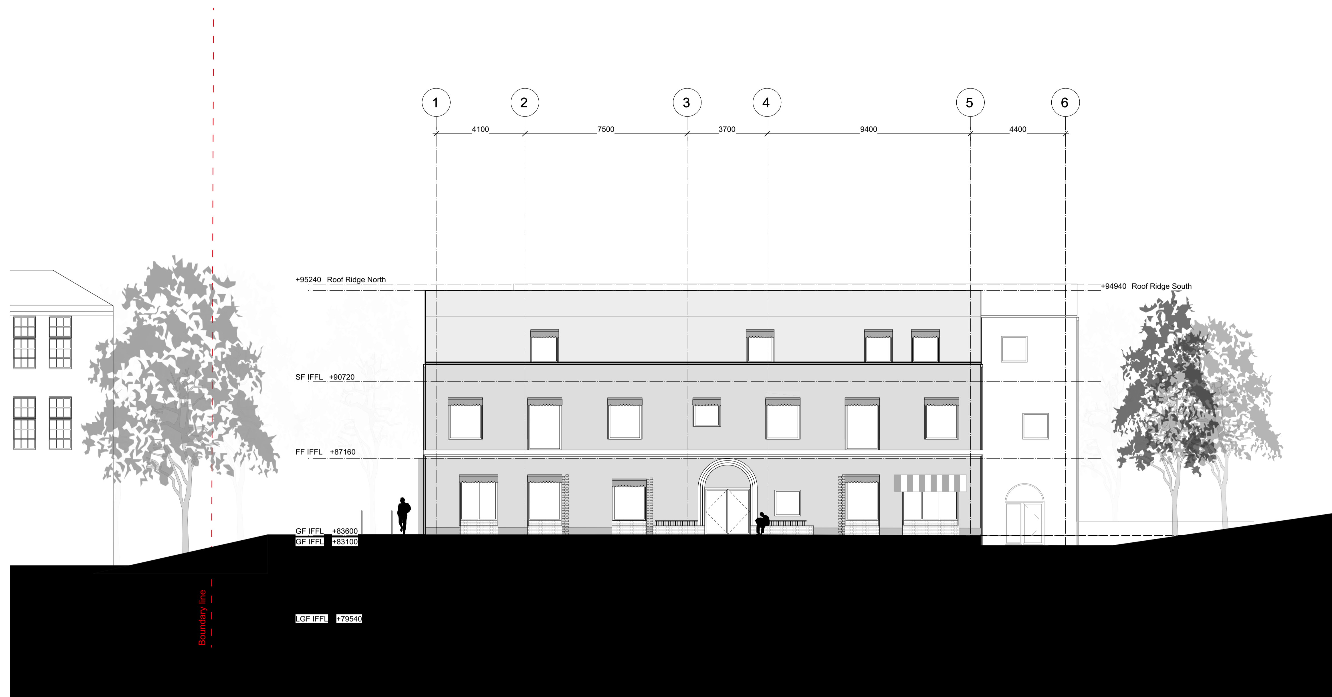
Building Elevation 1 - South
